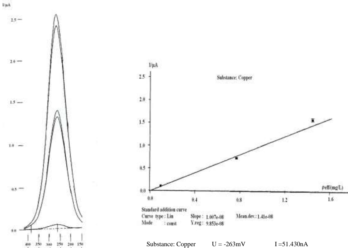
Fig. 3 Differential pulse polarogram and standard addition curve for Linseeds
